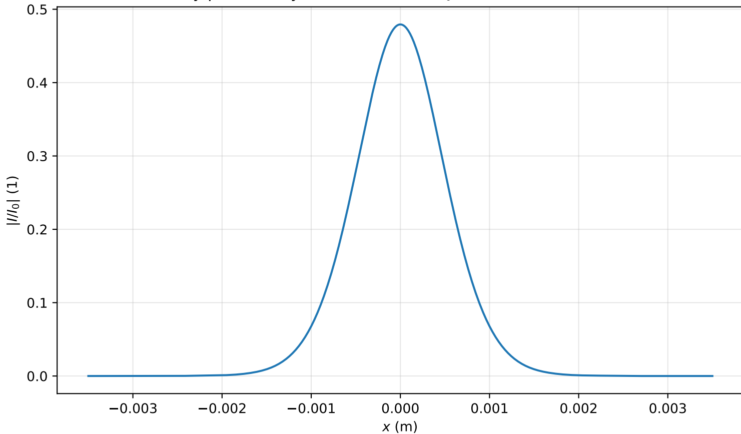
Intensity profile I(x, y = 0, z = 3.025m)/I_0 , P_{in}=0.4P_{cr} , artificial time
